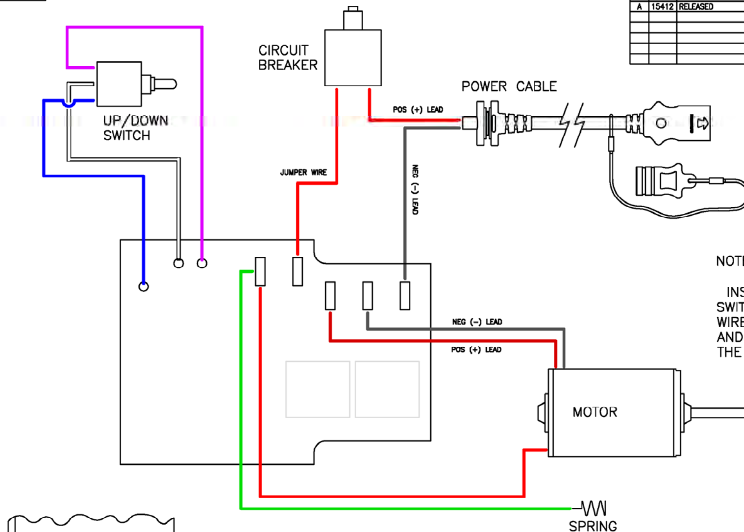
UP/DOWN SWITCH
