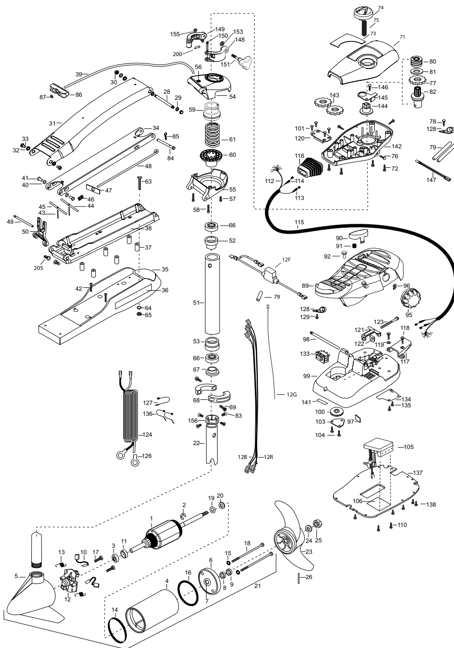
PARTS DIAGRAM
