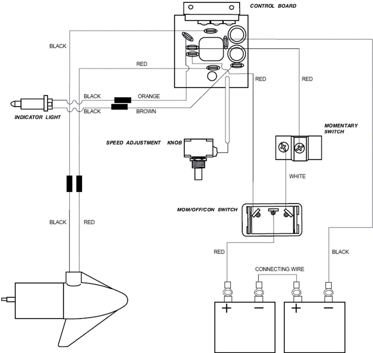
MAXXUM 65 Wiring Diagram
