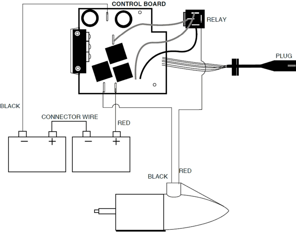
Wiring Diagram
