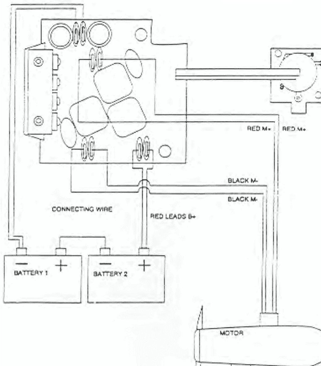
Wiring Diagram
