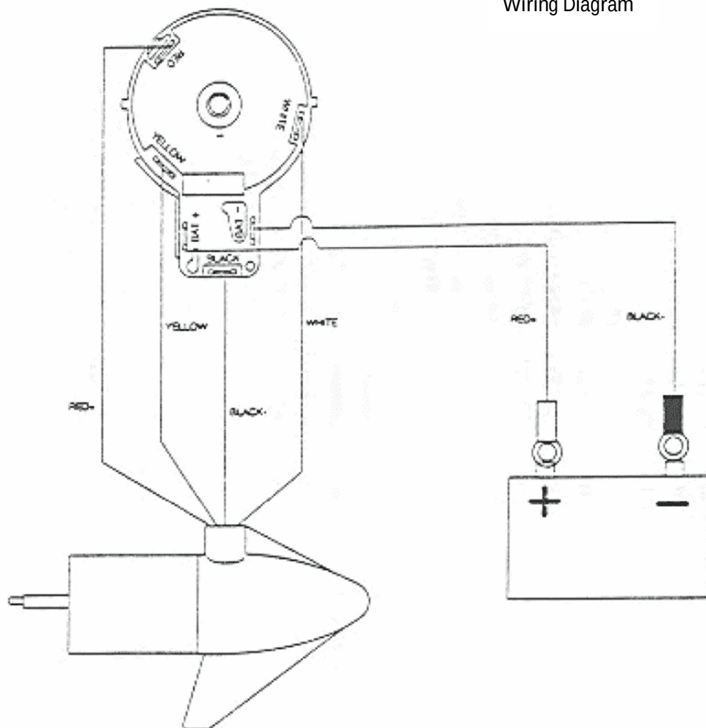
Wiring Diagram
