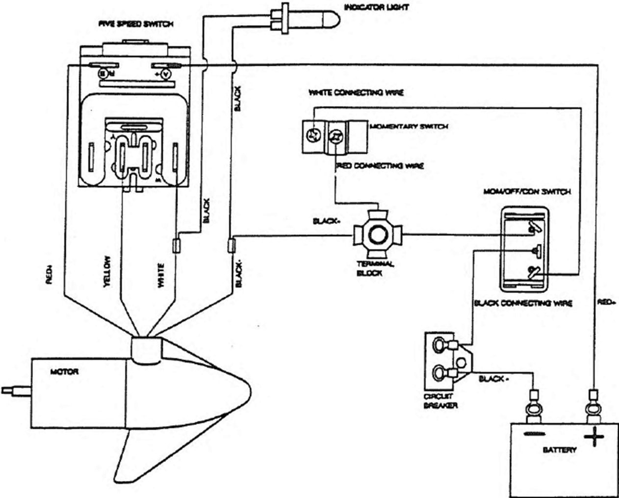
Wiring Diagram
