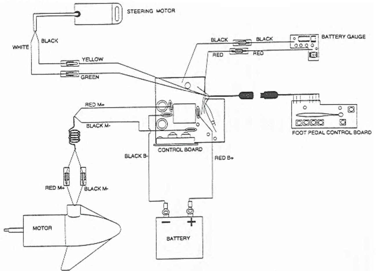
Wiring Diagram
