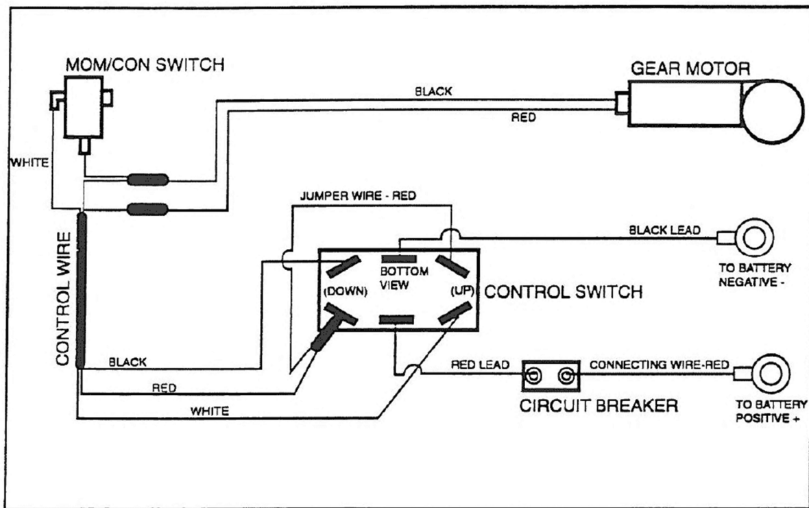
Wiring Diagram
