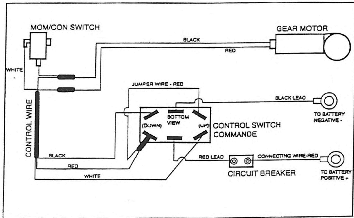
Wiring Diagram
