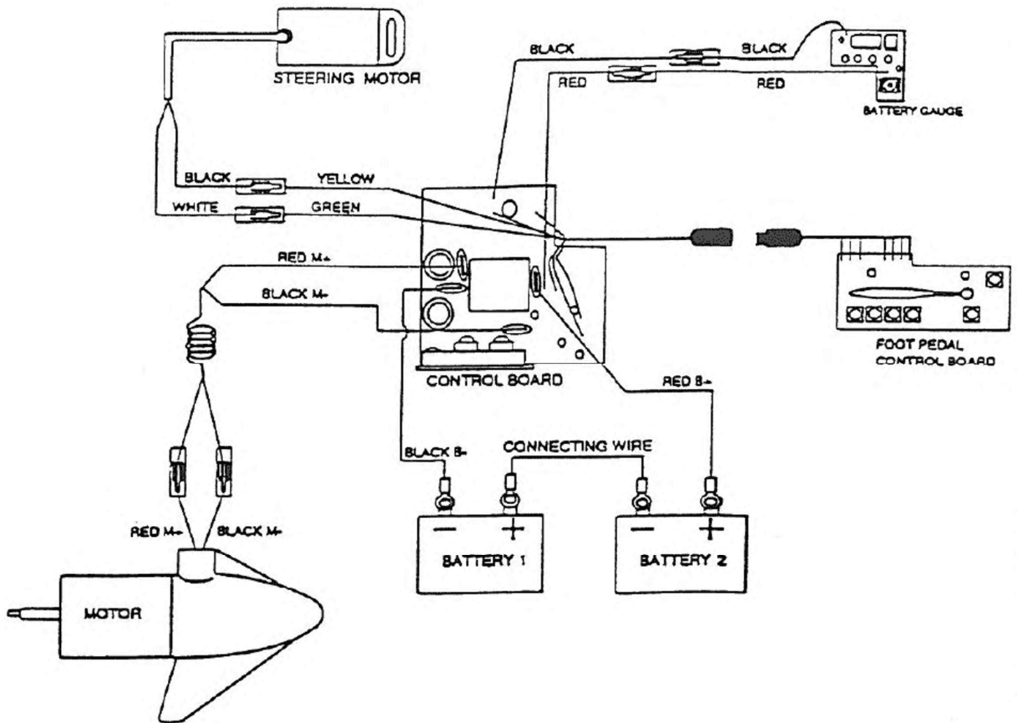
Wiring Diagram
